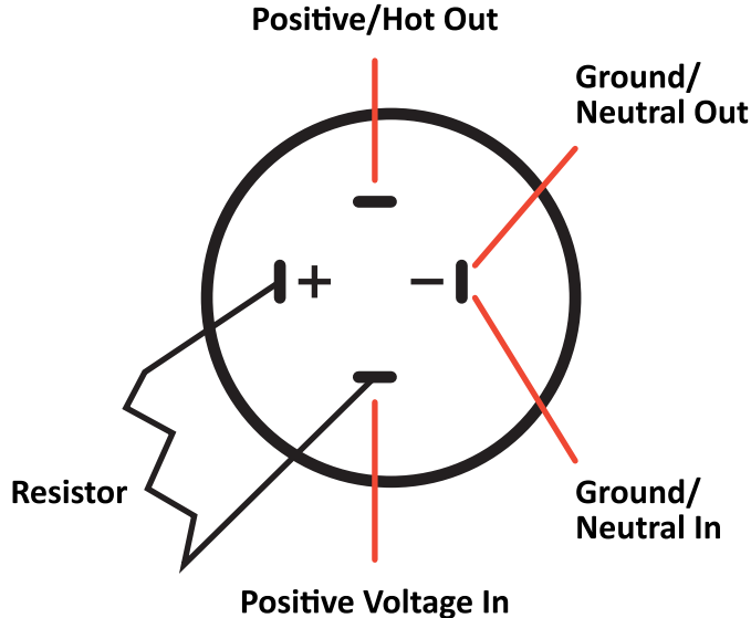
Switch Light Always On
