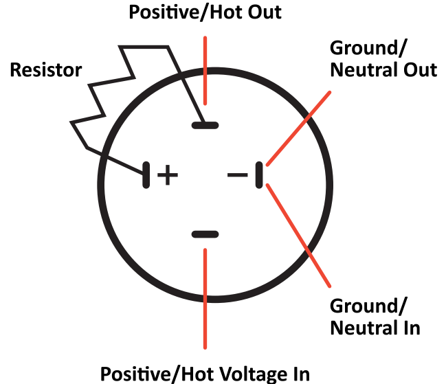
Switch Light Only On When Switch Is Activated
